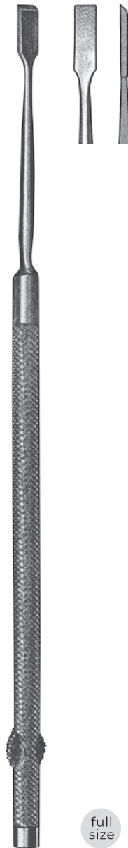
FREER Lachrymal Sac Chisels 4mm wide, straight, 16cm 33503.16
